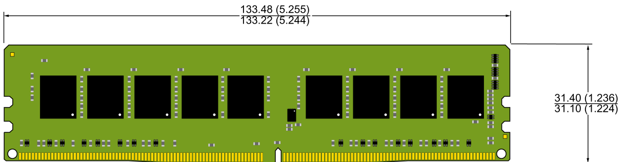
U-DIMM ECC MO-309 288 PIN
