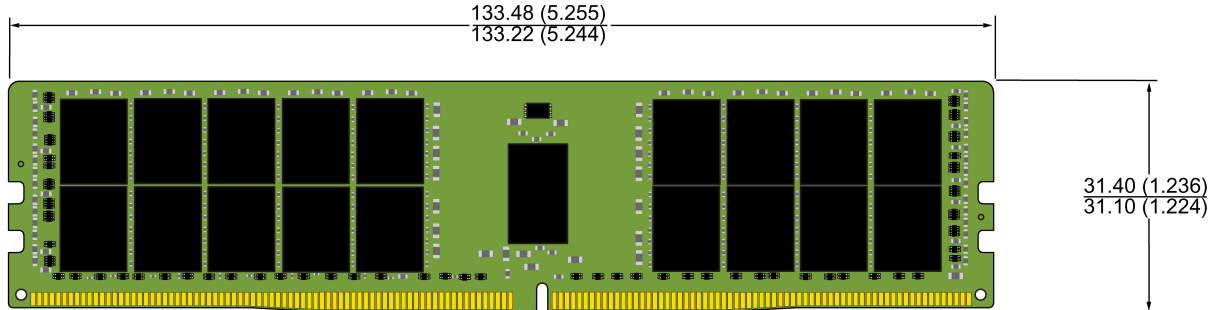
R-DIMM MO-309 288 PIN
