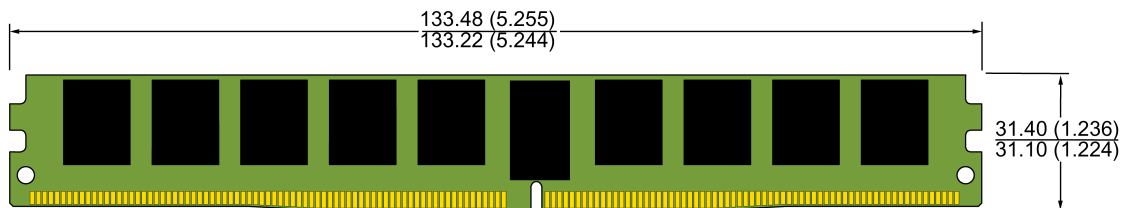
VLP R-DIMM MO-309 288 PIN
