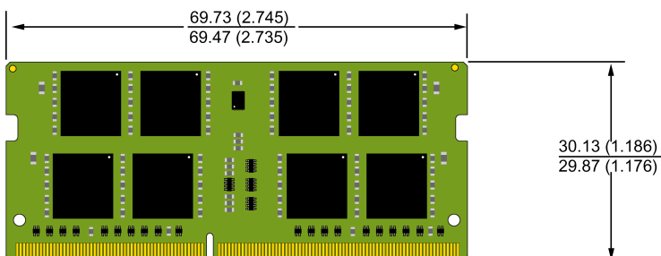
SO-DIMM MO-310 260 PIN
