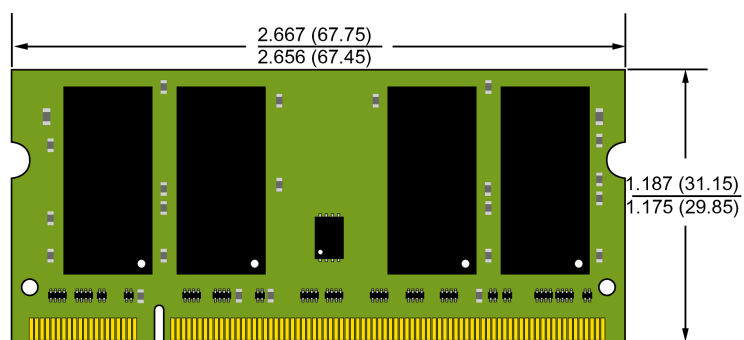
SO-DIMM MO-224 200 PIN
