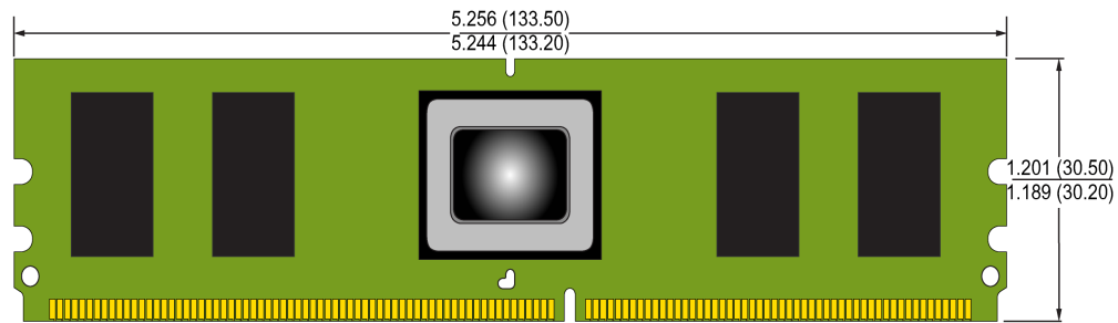
FB-DIMM MO-256 240 PIN
