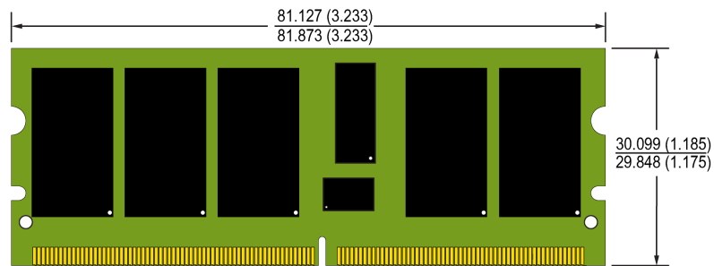
MINI-UDIMM MO-244 244 PIN
