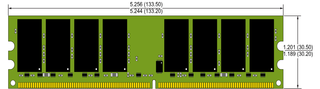
UDIMM MO-237 240 PIN
